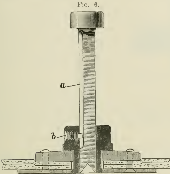
Section of Kögler's slaughter mask. a , groove for the bolt: b , screw for preventing the bolt from springing out.
